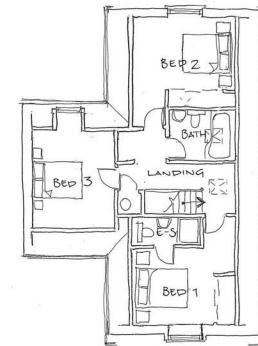
PLOT 2 FIRST FLOOR ~ 1:100
